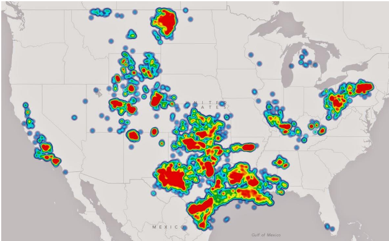
Fig. 3.2 Map of oil & natural gas drilling in the US, 2016, red and yellow colour means high and blue and green colour means lower intensities, according to ArcGIS-data from 2016 26
